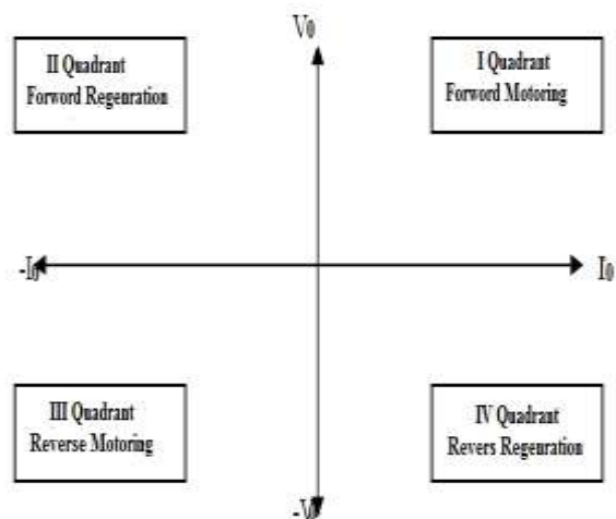
Basic operation of Four quadrant chopper
