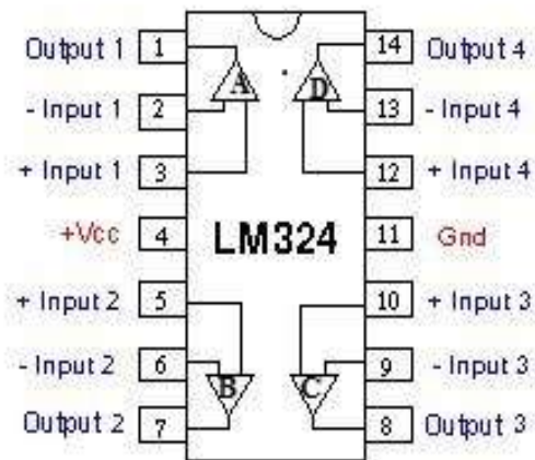
Fig 3:- Pin Diagram of LM324
