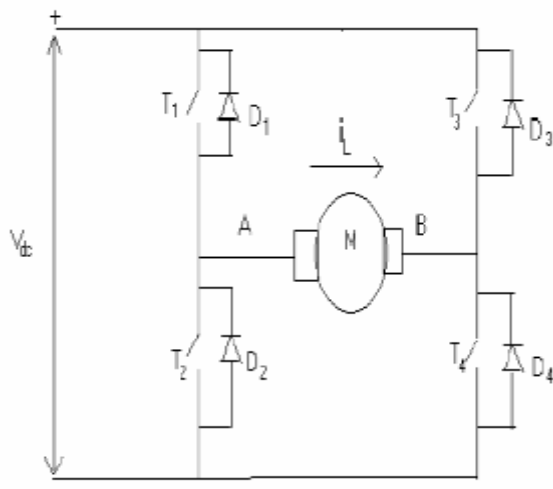
Fig1 :-Four quadrant chopper circuit
